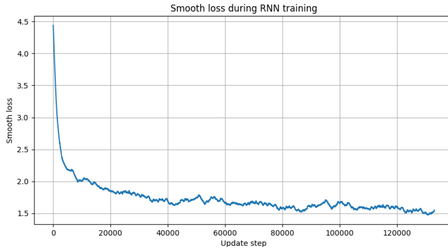
Figure 1: Smooth loss function over 133000 update steps ( \sim 3 epochs)
